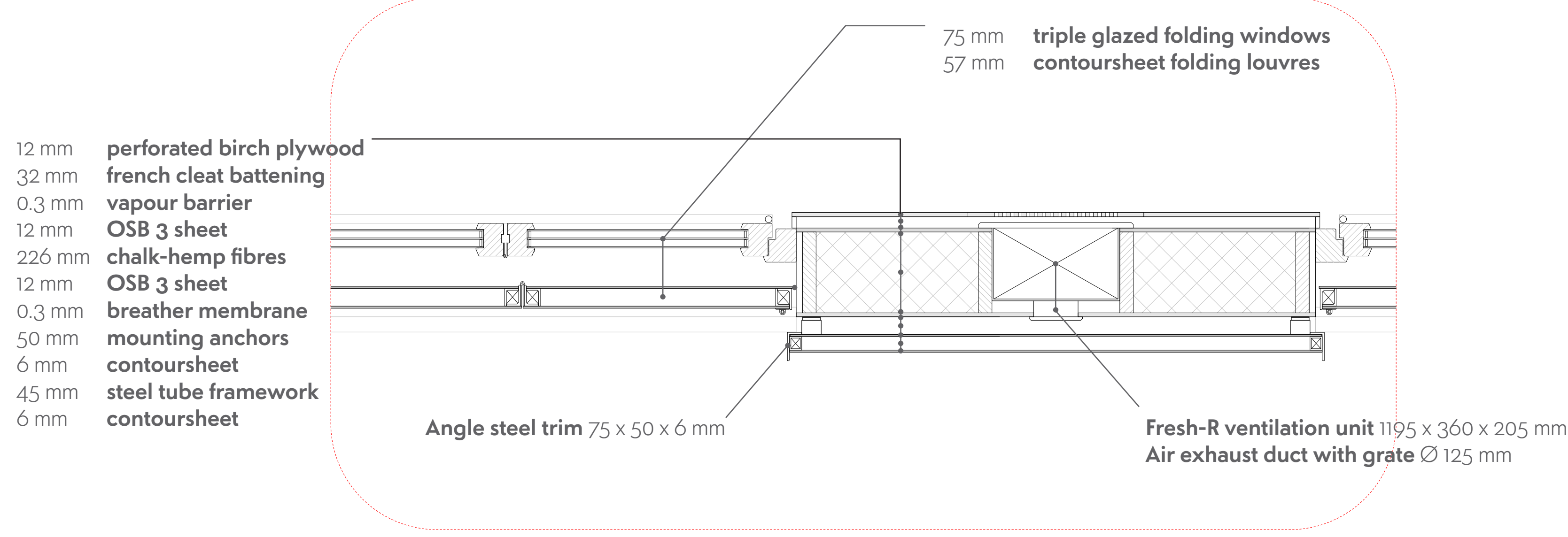
Horizontal detail 1:10
